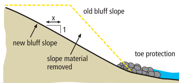
Cutback Slope Stabilization Method
