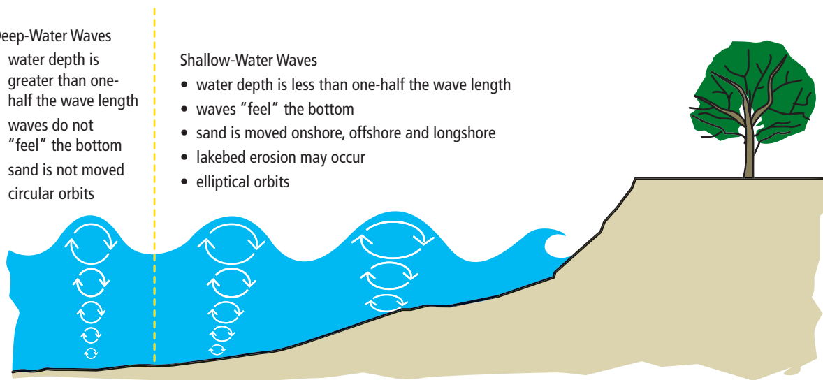
Waves Feeling the Lake Bottom
