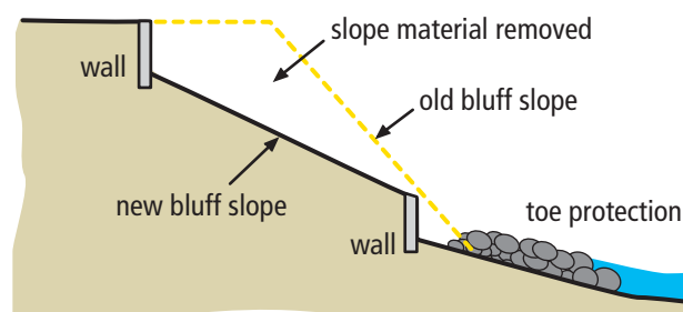
Terraced Bluff Stabilization Method
