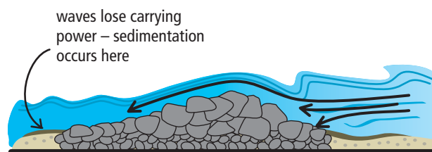
Tripping Waves (Submerged Breakwater)
