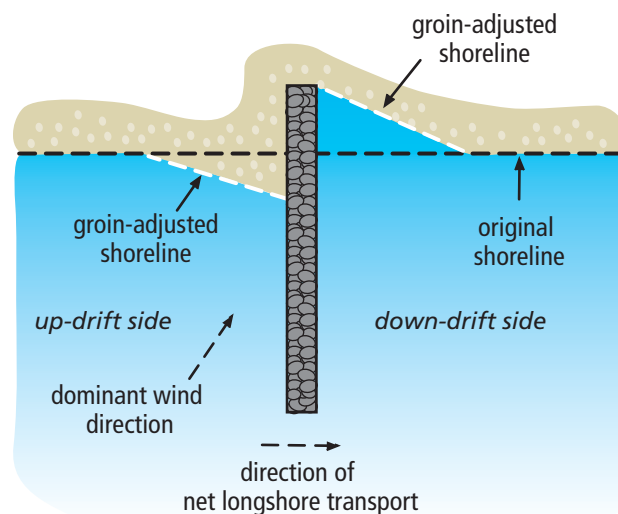
Beach Response to a Groin
