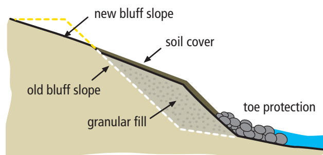
Cut and Fill Slope Stabilization Method
