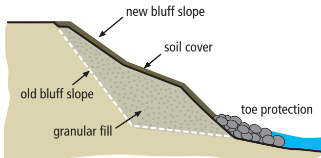
Fill Slope Stabilization Method
