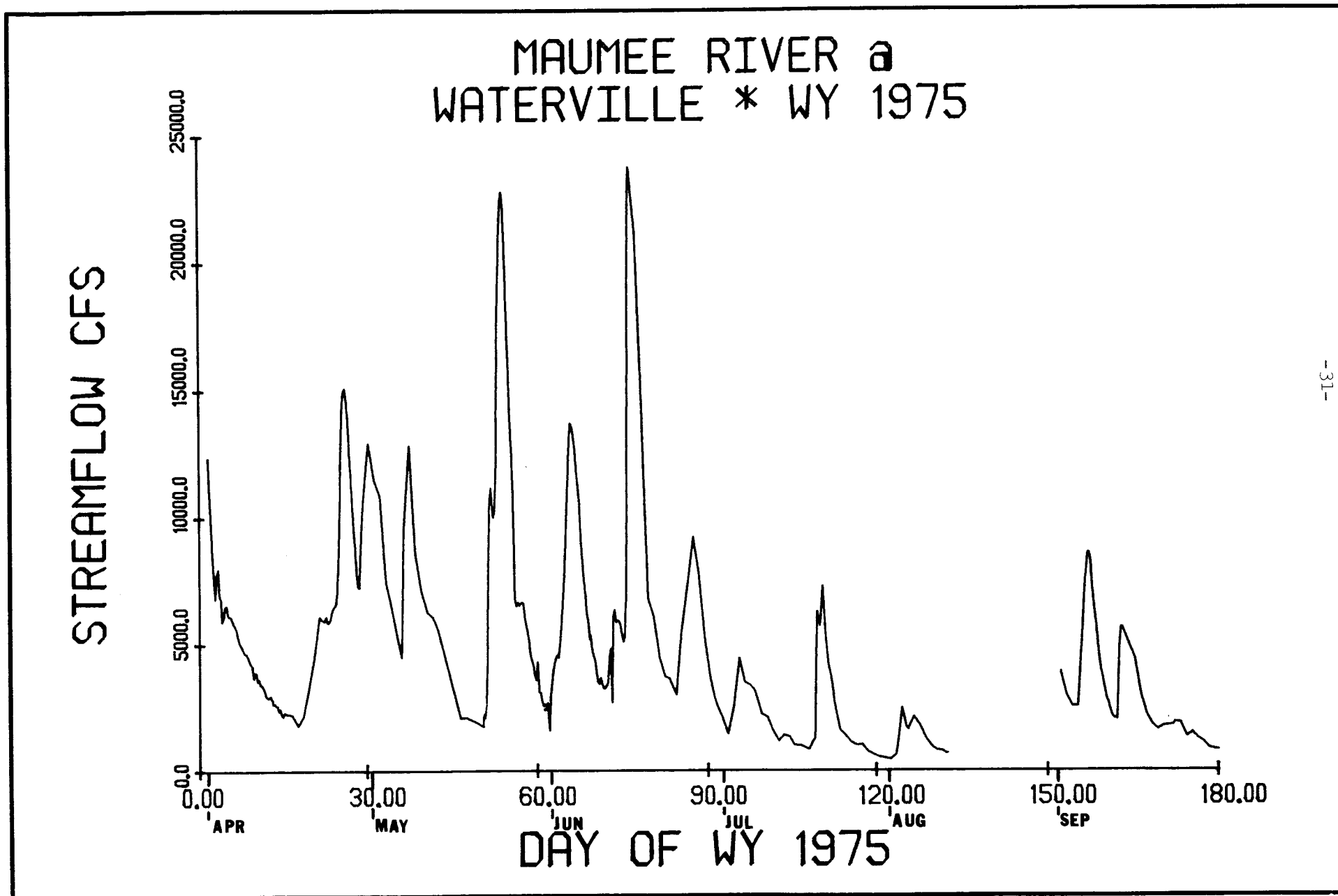
Figure 4. Flow hydrographs for Maumee River at Waterville, 1975.
