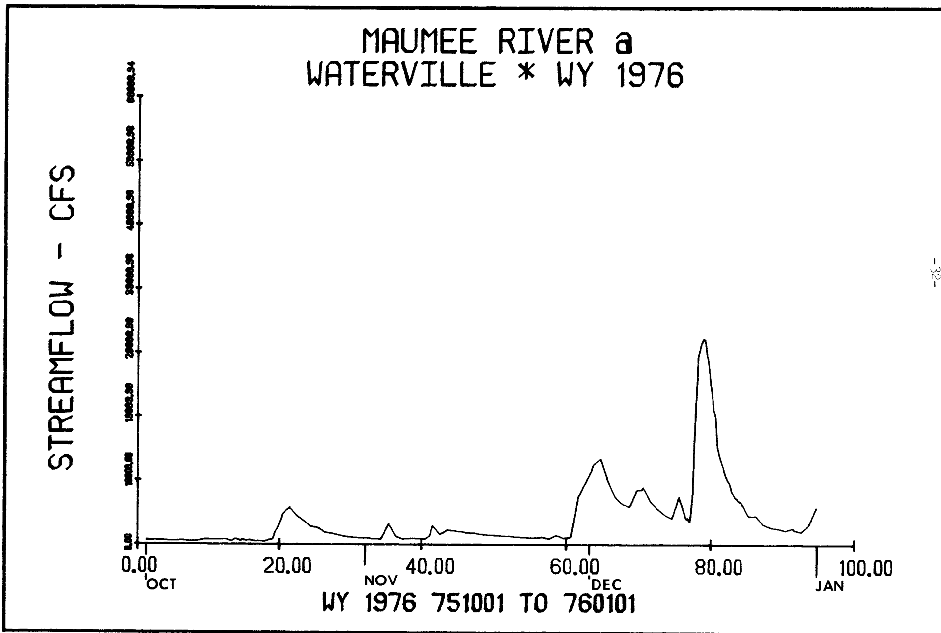
Figure 5. Flow hydrographs for Maumee River at Waterville, 1976.
