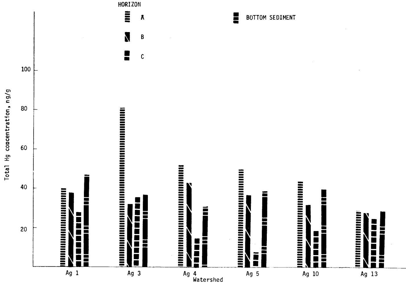
Fig. 4. Total mercury concentration of soil and bottom sediment for agricultural watersheds. Values weighted from area occupied by each soil series within each watershed.
