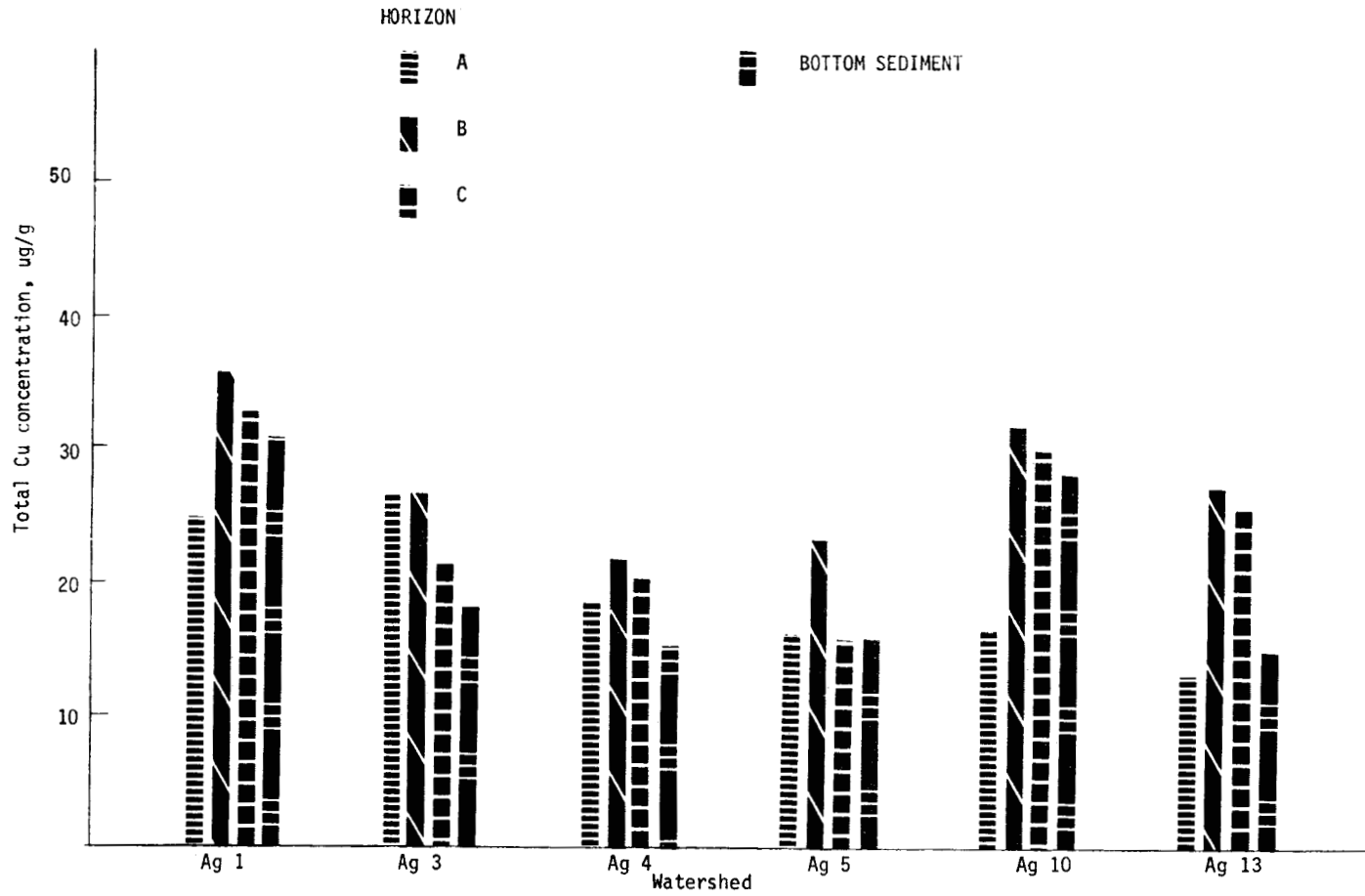
Fig. 3. Total copper concentration of soil and bottom sediment for agricultural watersheds. Values weighted from area occupied by each soil series within each watershed.
