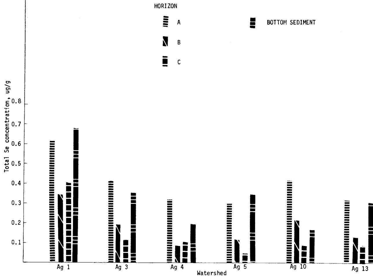
Fig. 8. Total selenium concentration of soil and bottom sediment for agricultural watersheds. Values weighted from area occupied by each soil series within a watershed.
