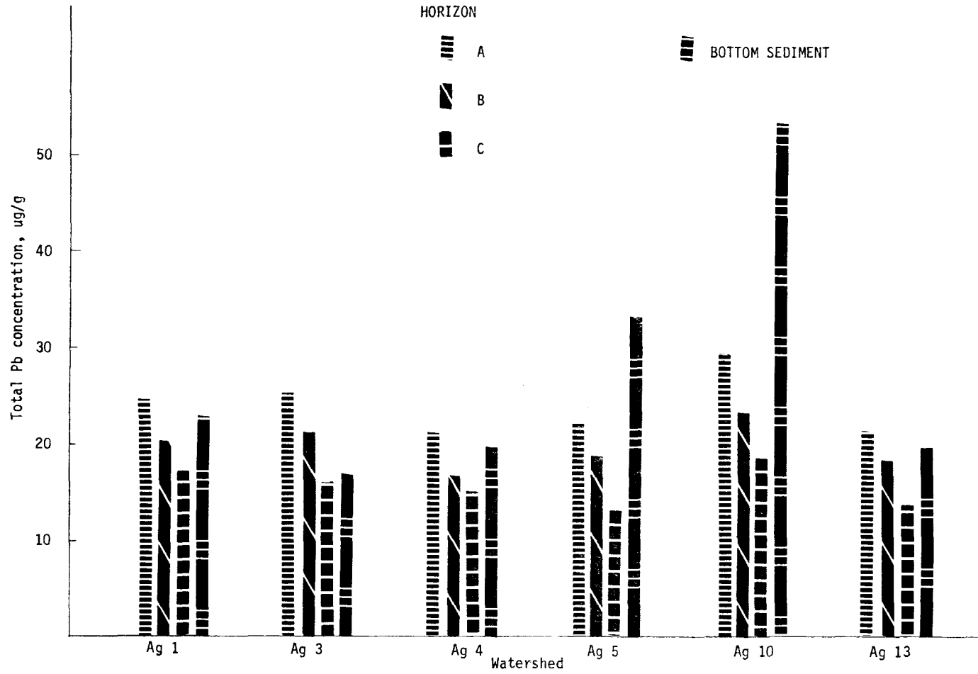
Fig. 7. Total lead concentration of soil and bottom sediment for agricultural watersheds. Values weighted from area occupied by each soil series within a watershed.
