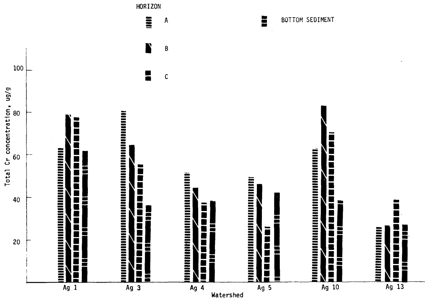
Fig. 2. Total chromium concentration of soil and bottom sediment for agricultural watersheds. Values weighted from area occupied by each soil series within each watershed.
