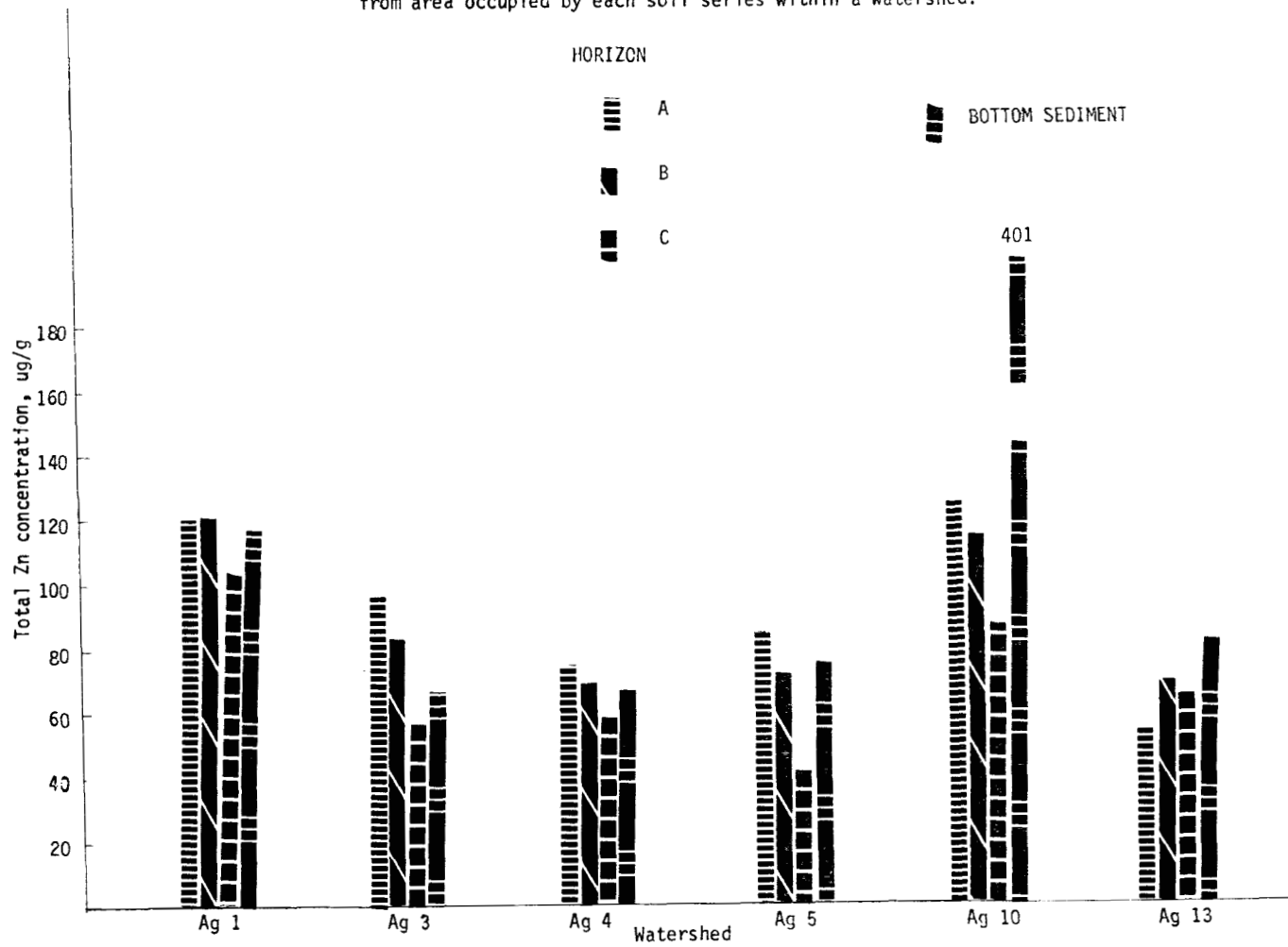
Fig. 9. Total zinc concentration of soil and bottom sediment for agricultural watersheds. Values weighted from area occupied by each soil series within a watershed.
