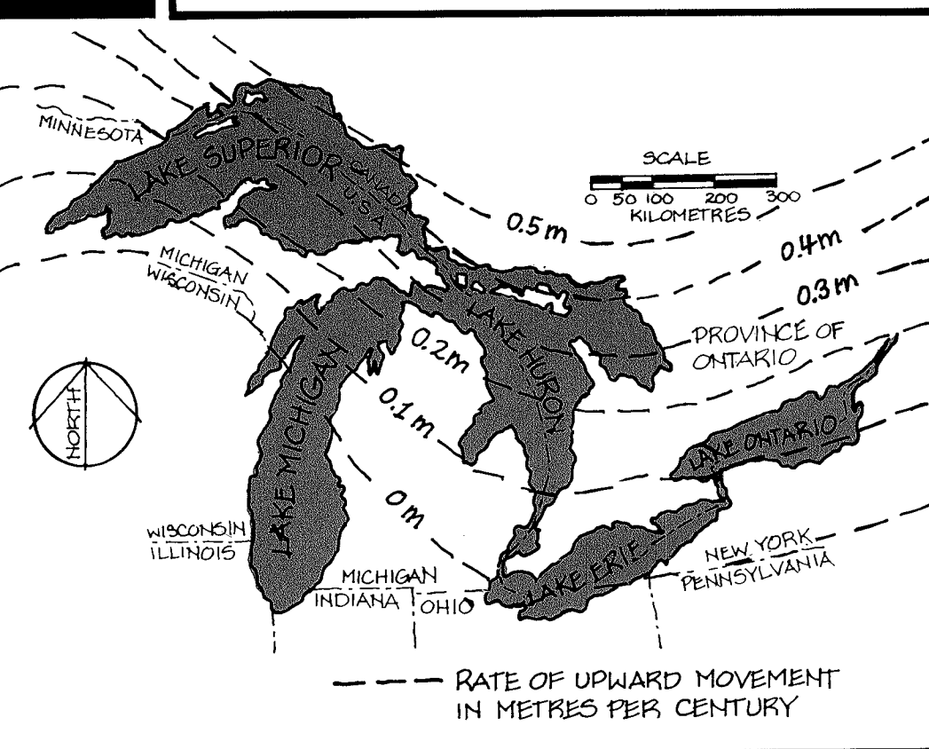
CRUSTAL MOVEMENT
